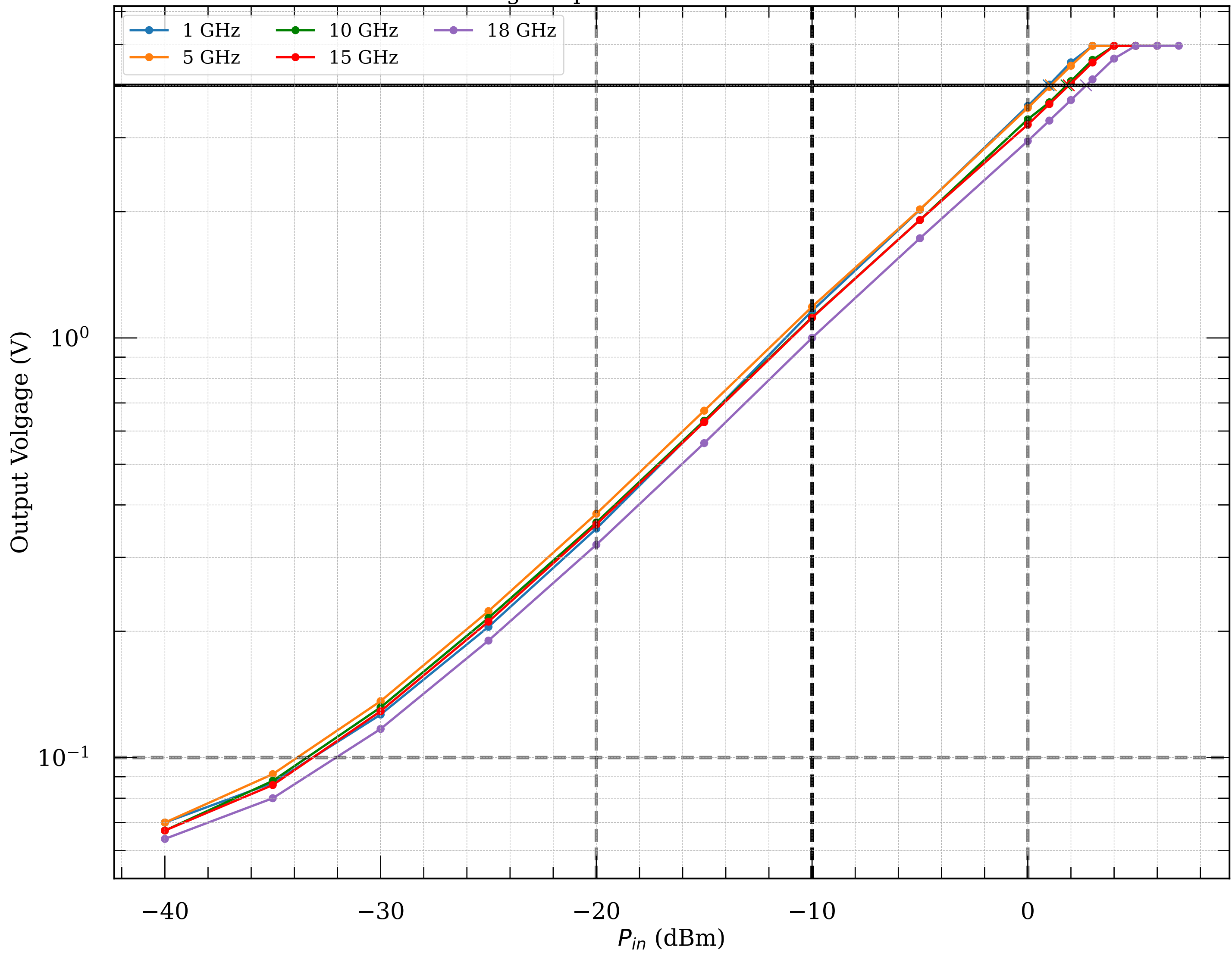
Measured voltage-to-power curve of detector module021v2
